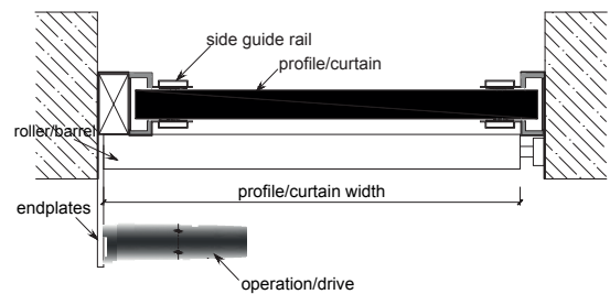
Plan at Roller/Barrel Level
