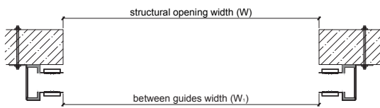
Plan at Guide Level
