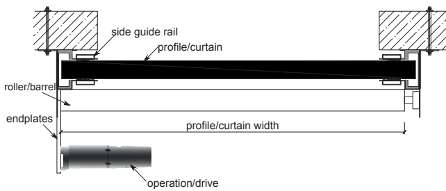
Plan at Roller/Barrel Level
