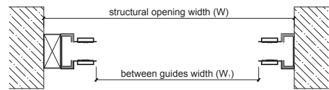
Plan at Guide Level
